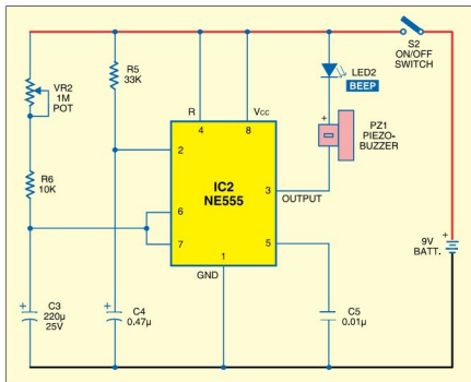
Fig. 2: Timer circuit
