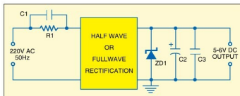
Fig. 1: Suggested circuit for a transformerless DC power supply
