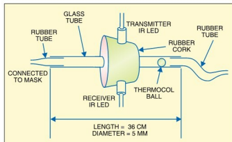
Fig. 6: Physical interface assembly for respiration rate measurement
