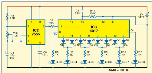
Fig. 3: Circuit for LED pendulum
