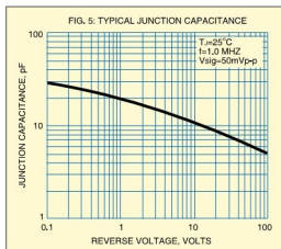
Fig. 5: Performance curves of diodes 1N4001 to 1N4007
