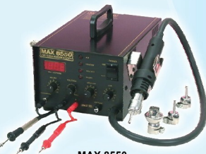
MAX 8550 SMD REWORK STATION THREE IN ONE • Hot Air Soldering De-soldering • Micro Soldering Station • 1.2 VDC-18 VDC Digital Regulated Power Station
