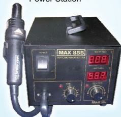
MAX 855 UPGRADE model: A fully automatic Soldering Station with "Digital air temperature controller" for accurate soldering-desoldering
