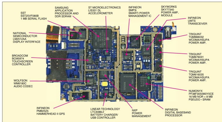
Fig. 2: Logic board of iPhone 3G showing the different ICs used
