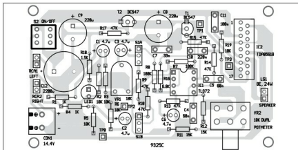
Fig. 3: Component layout for the PCB
