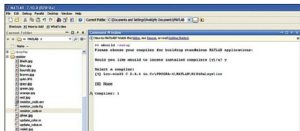
Fig. 4: mbuild setup command
