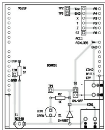
Fig. 3: Component layout for the PCB
