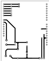
Fig. 2: An actual-size PCB layout for the sequential tilt-motion lock
