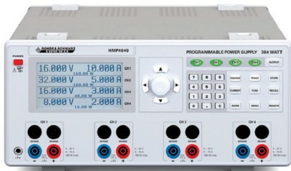
Rohde &amp; Schwarz HMP4040 programmable four-channel power supply
