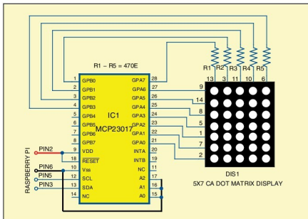
Fig. 12: Circuit diagram of 5x7 dot-matrix display
