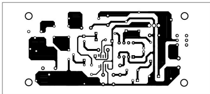
Fig. 2: An actual-size, single-side PCB for crystal-controlled single-frequency FM transmitter
