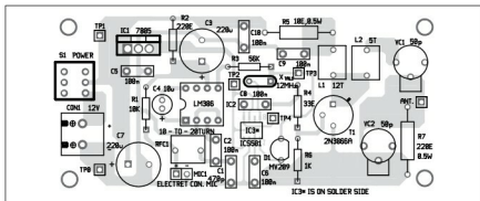
Fig. 3: Component layout for the PCB
