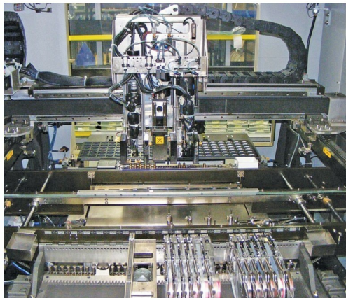
Pick-and-place internals of a surface mount machine (Courtesy: en.wikipedia.org)
