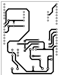
Fig. 4: An actual-size PCB layout for the circuit
