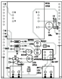
Fig. 5: Component layout for the PCB
