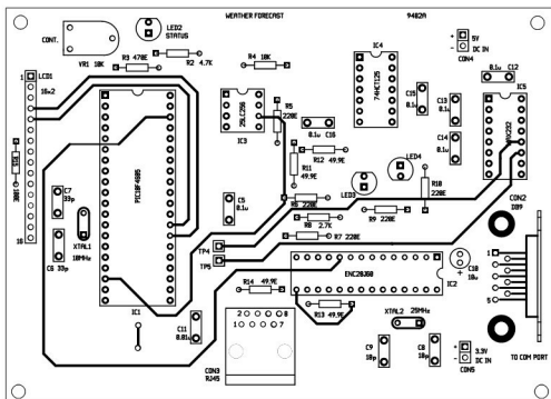
Fig. 7: Component-side track layout of the PCB
