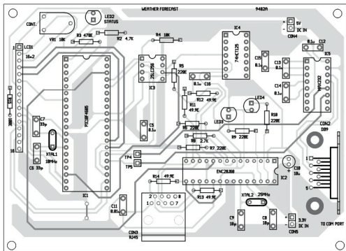
Fig. 8: Component layout of the client board circuit
