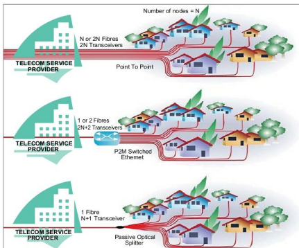
Fig. 6: P2P Ethernet, P2M switched Ethernet and PON
