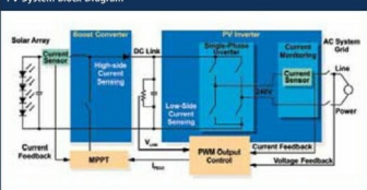
PV System Block Diagram
