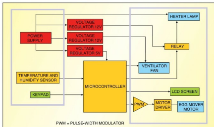
Block diagram of an electronic egg incubator
