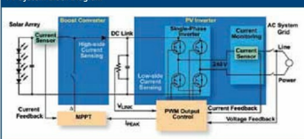
PV System Block Diagram
