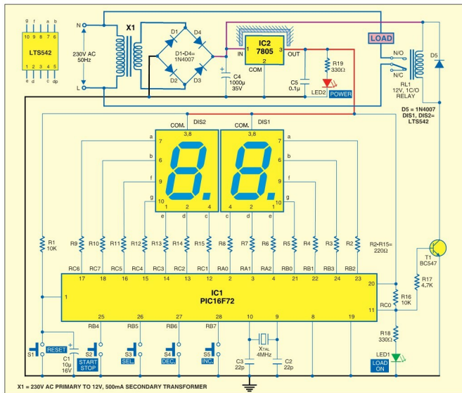
Fig. 1: Circuit of time-controlled switch using PIC16F72 microcontroller
