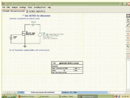
Fig. 4: DC device curves analysis in 5Spice
