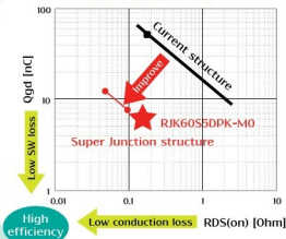
Performance Comparison Of Super Junction MOSFET
