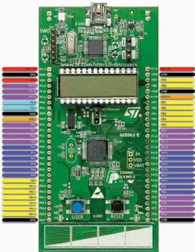
STMicroelectronics' STM32L Discovery board
