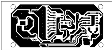
Fig. 3: An actual-size, single-side PCB for the automatic fan controller for ACs
