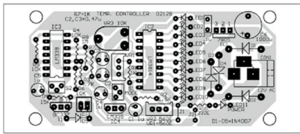
Fig. 4: Component layout for the PCB
