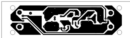
Fig. 4: An actual-size, single-side PCB for the live home security system
