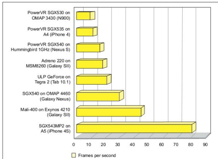
Fig. 3: GLBenchmark 2.1 Offscreen
