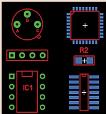
Fig. 5: Sprint-Layout components library
