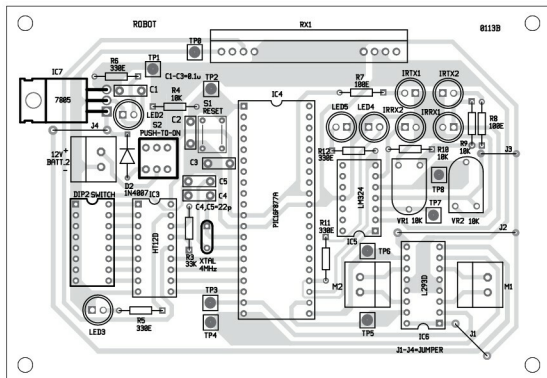
Fig. 8: Component layout for the PCB in Fig. 7
