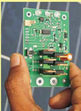
Solar Charger 24V/30A
