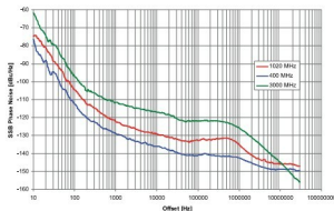
SSB Phase Noise
