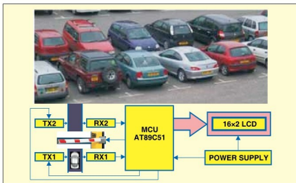
Fig. 1: Block diagram of automatic car parking space management system
