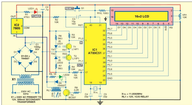
Fig. 2: Circuit for automatic car parking space management system
