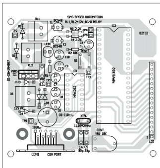
Fig. 3: Component layout for the PCB
