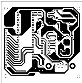
Fig. 2: Actual-size, single-side PCB for the SMS-based automation system
