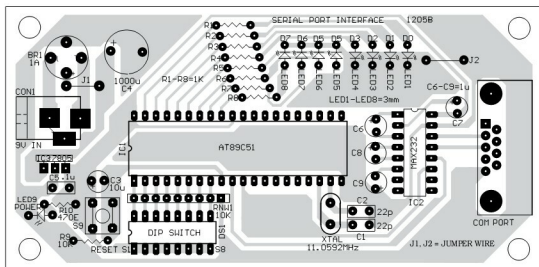
Fig. 6: Component layout for the PCB
