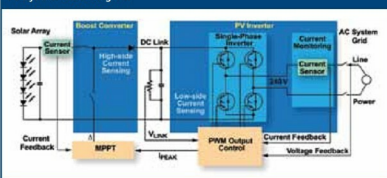
PV System Block Diagram
