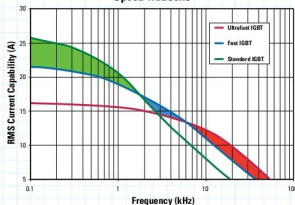
Speed Tradeoffs
