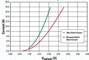
Short Circuit vs Efficiency Tradeoff
