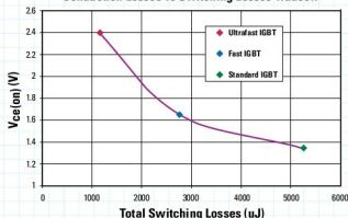
Conduction Losses vs Switching Losses Tradeoff
