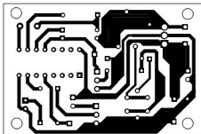
Fig. 2: An actual-size, single-side PCB for sensitive LPG sensor
