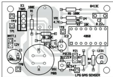
Fig. 3: Component layout for the PCB
