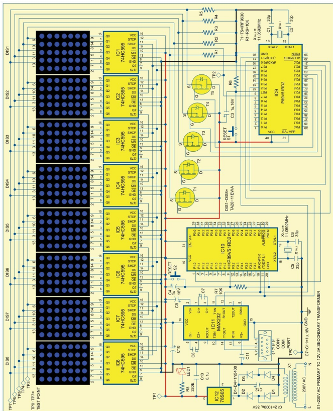
Fig. 3: Circuit of GSM-based dot-matrix display
