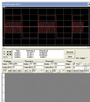
Fig. 2: Simulation results for the circuit on National Instruments' circuit suite
