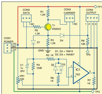
Fig. 3: Circuit for ASK communication trainer
