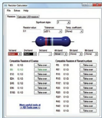
Fig 1: Home screen of resistor calculator
