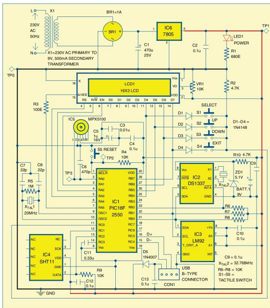
Fig. 2: Circuit diagram of a weather logger
