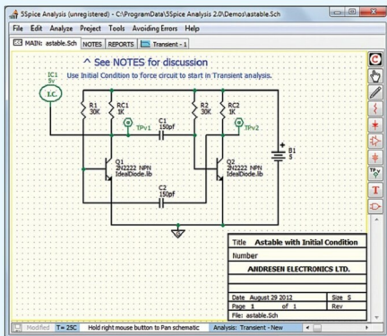
Fig. 2: Demo schematic of astable circuit
