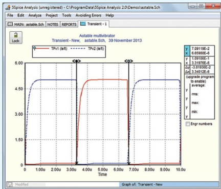
Fig. 3: Transient analysis graph of astable circuit
