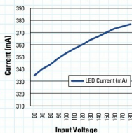
IRPLLED7 Demo Board LED Current vs Input Voltage
