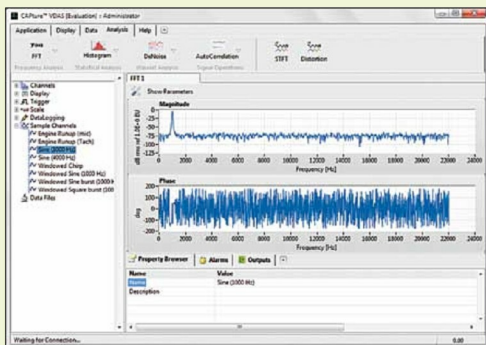
Fig. 2: FFT Analysis
