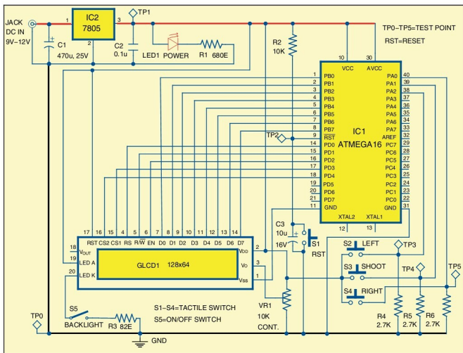
Fig. 3: Circuit of Space Invaders hand video game
