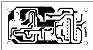
Fig. 2: An actual-size, single-side PCB for the touch alarm
