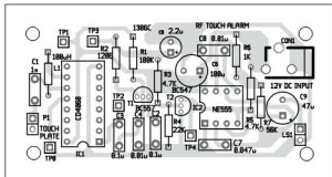
Fig. 3: Component layout for the PCB
