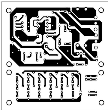
Fig. 2: An actual-size, single-side PCB for the simple manual PWM generator
