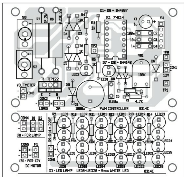
Fig. 3: Component layout for the PCB
