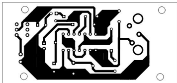
Fig. 3: An actual-size, single-side PCB for bedwetting alarm
