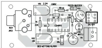
Fig. 4: Component layout for the PCB
