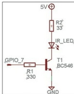
Fig. 13: IR circuit for remote control
