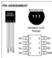
Fig. 11: DS18B20 pin configurations
